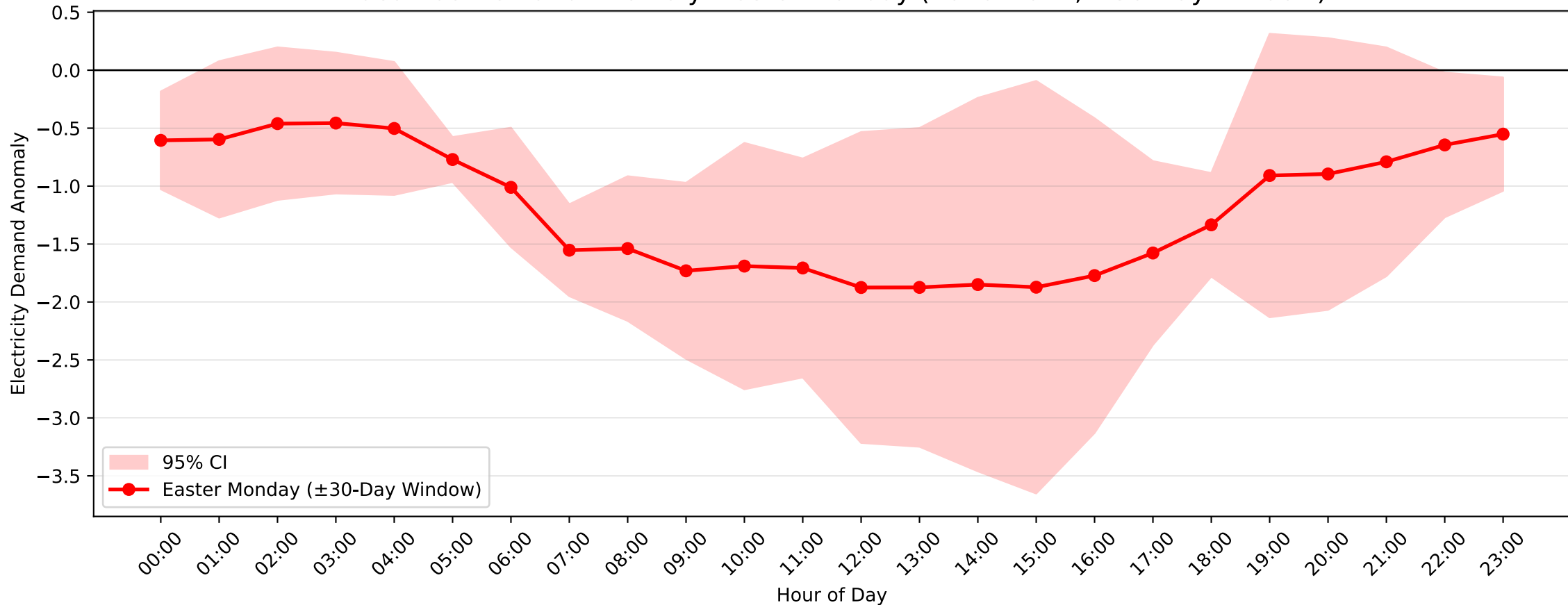
Lidcombe Demand Anomaly: Easter Monday (2016–2017, \pm 30 -Day Window)
