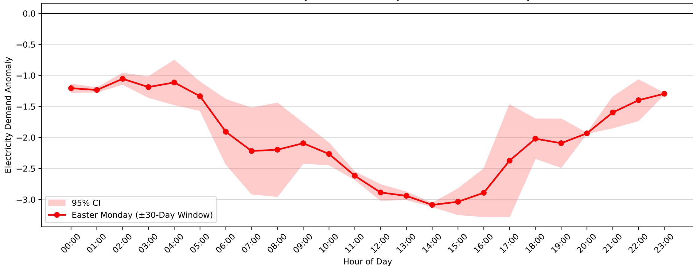
Lidcombe Demand Anomaly: Easter Monday (2009–2010, \pm 30 -Day Window)
