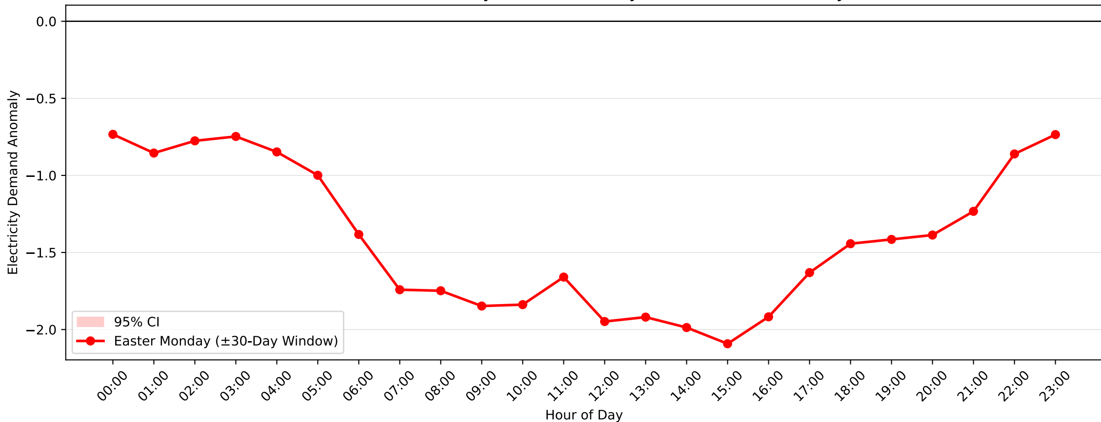
Lidcombe Demand Anomaly: Easter Monday (2017-2018, \pm 30 -Day Window)
