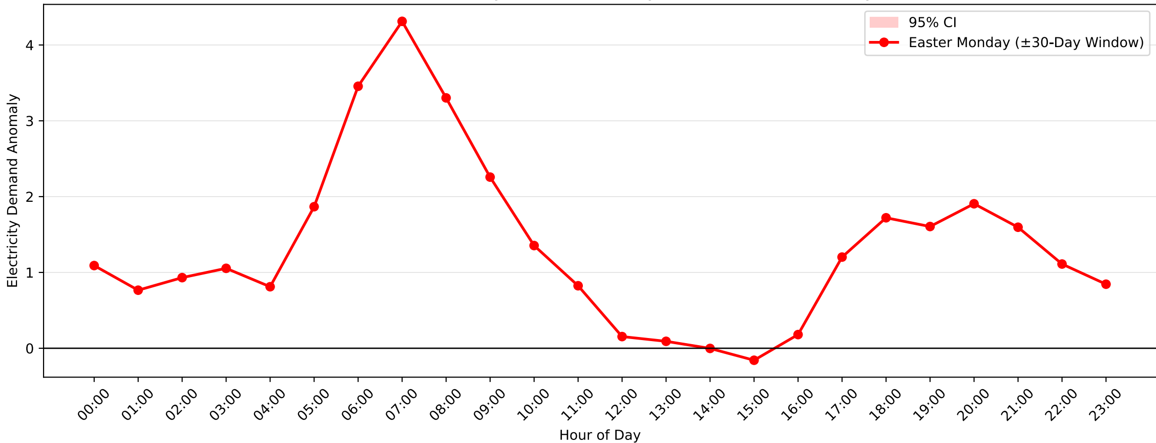
Lidcombe Demand Anomaly: Easter Monday (2004–2005, \pm 30 -Day Window)
