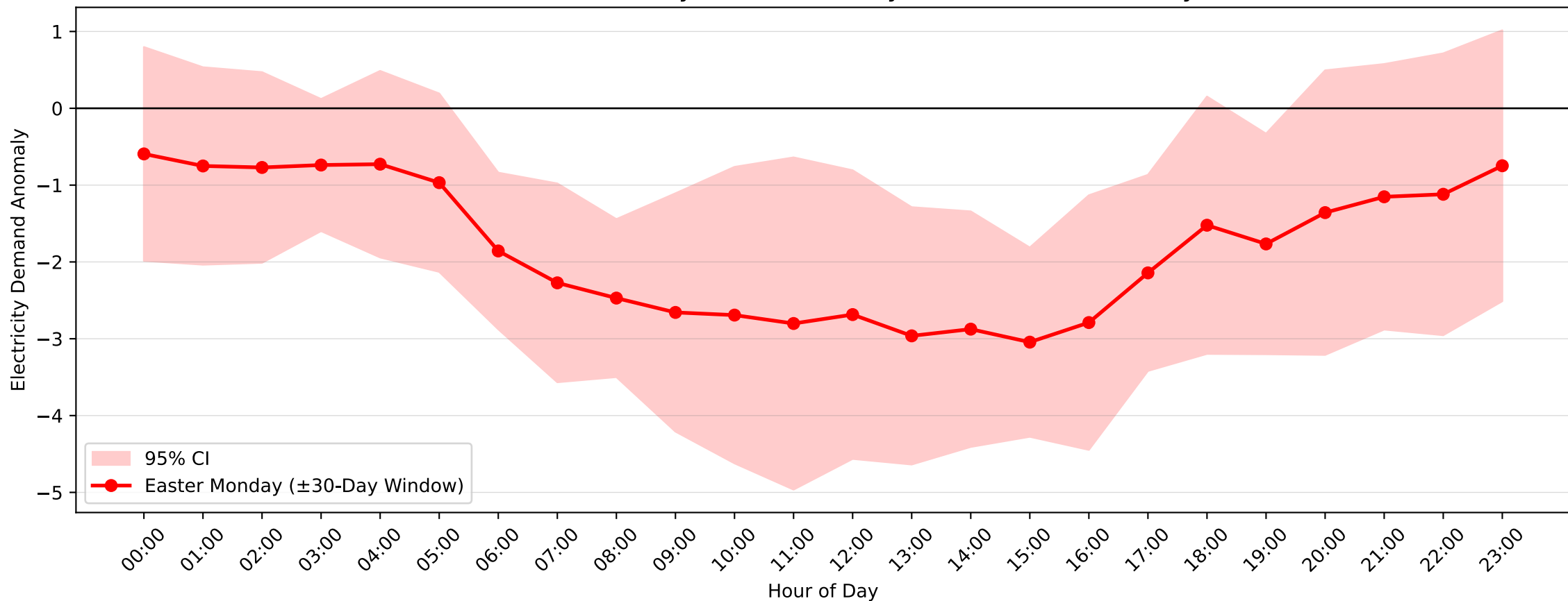
Lidcombe Demand Anomaly: Easter Monday (2006–2007, \pm 30 -Day Window)
