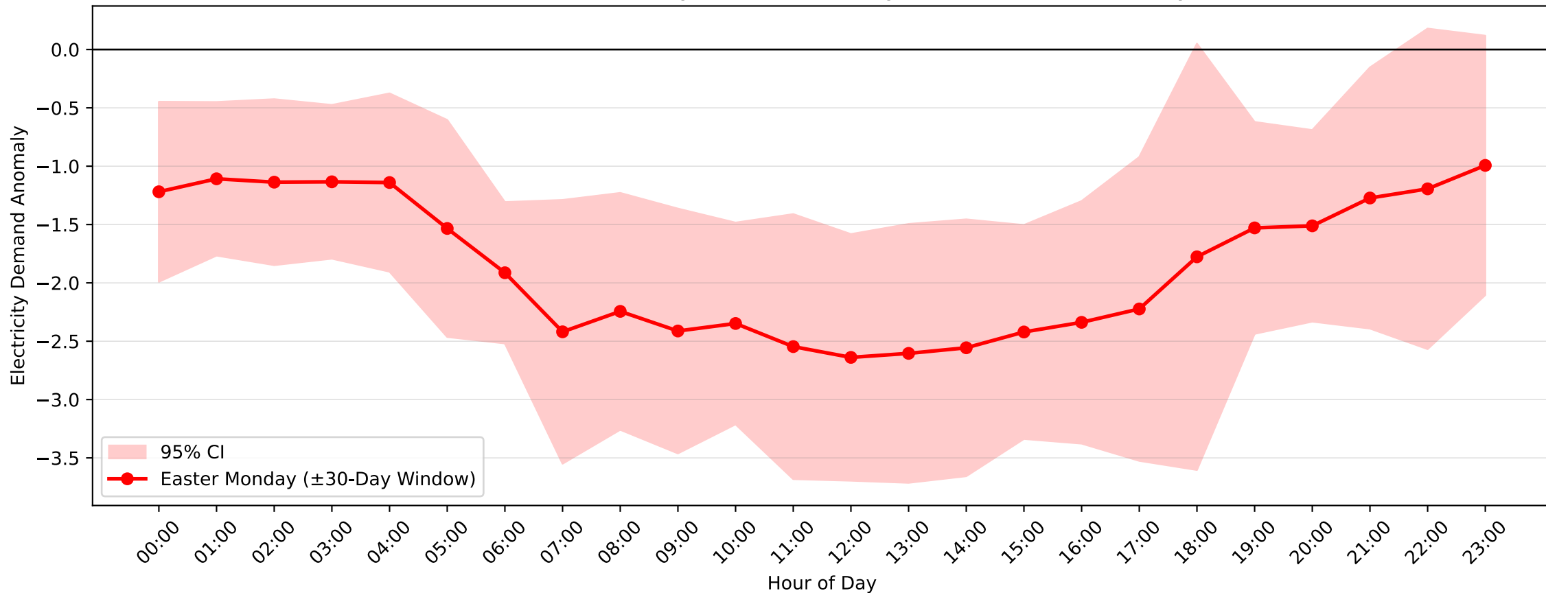
Lidcombe Demand Anomaly: Easter Monday (2012-2013, \pm 30 -Day Window)
