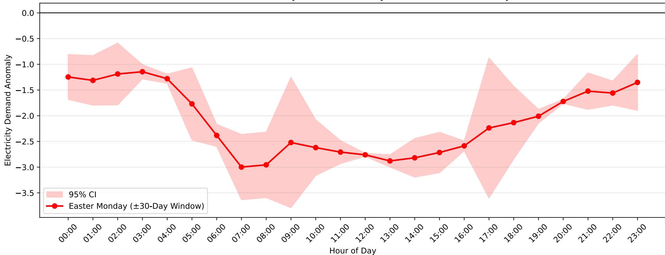
Lidcombe Demand Anomaly: Easter Monday (2008–2009, \pm 30 -Day Window)
