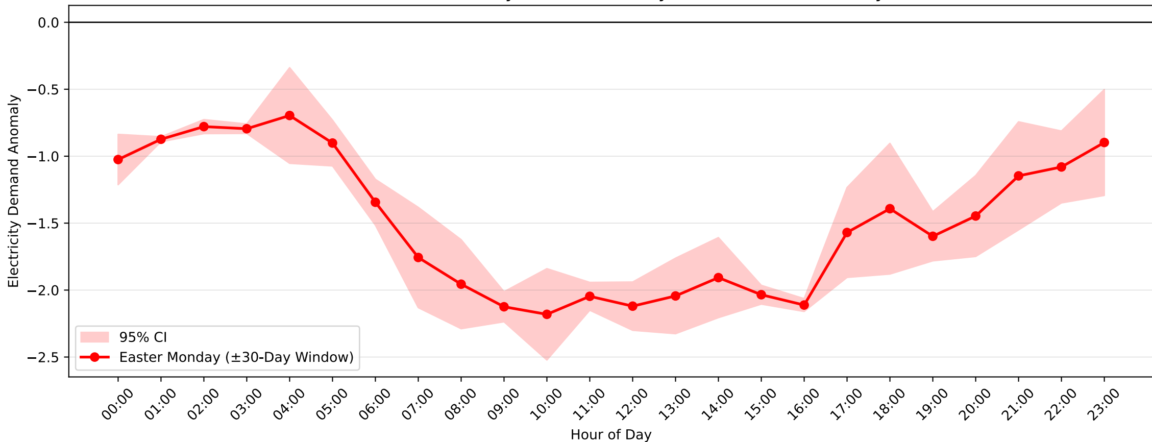
Lidcombe Demand Anomaly: Easter Monday (2014-2015, \pm 30 -Day Window)
